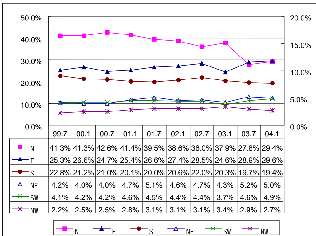
Figure1-8 Geographic Distribution of CN Domain Names
