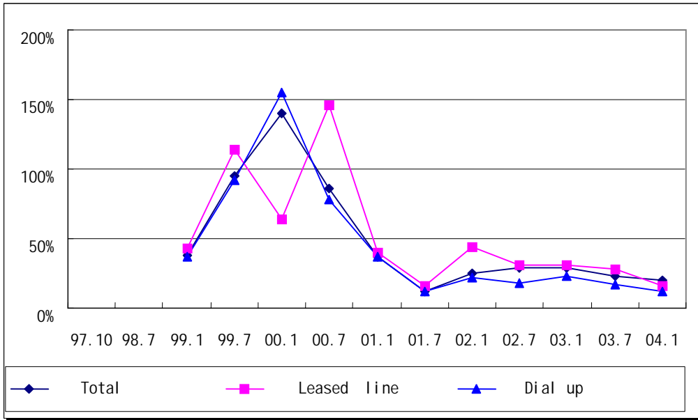
Figure 1-3 The growth rate of computer host
