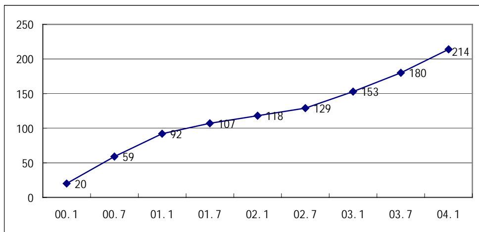
Figure3-4 Number of users who use other Internet accessing facilities ( in ten thousand )
