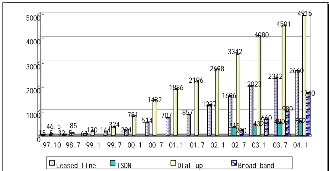
Figure1-5 Users of different accessing methods (in 10 thousand)
