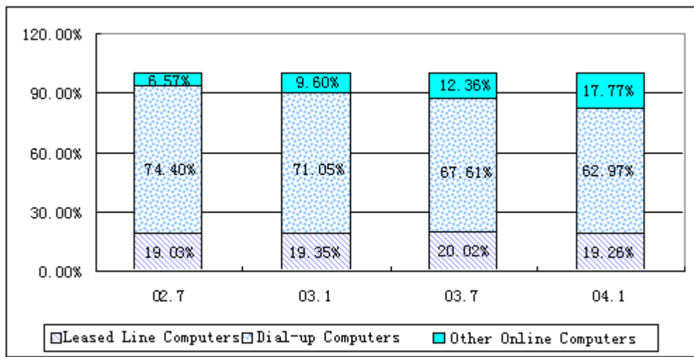
Figure3-11 Proportion of computer hosts in different connecting ways
